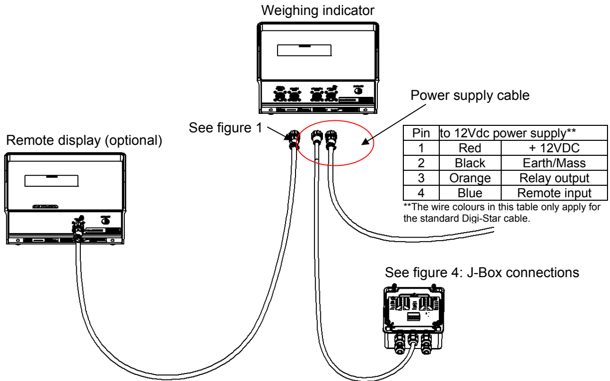
Figure 2: Connection diagram of weighing indicator
