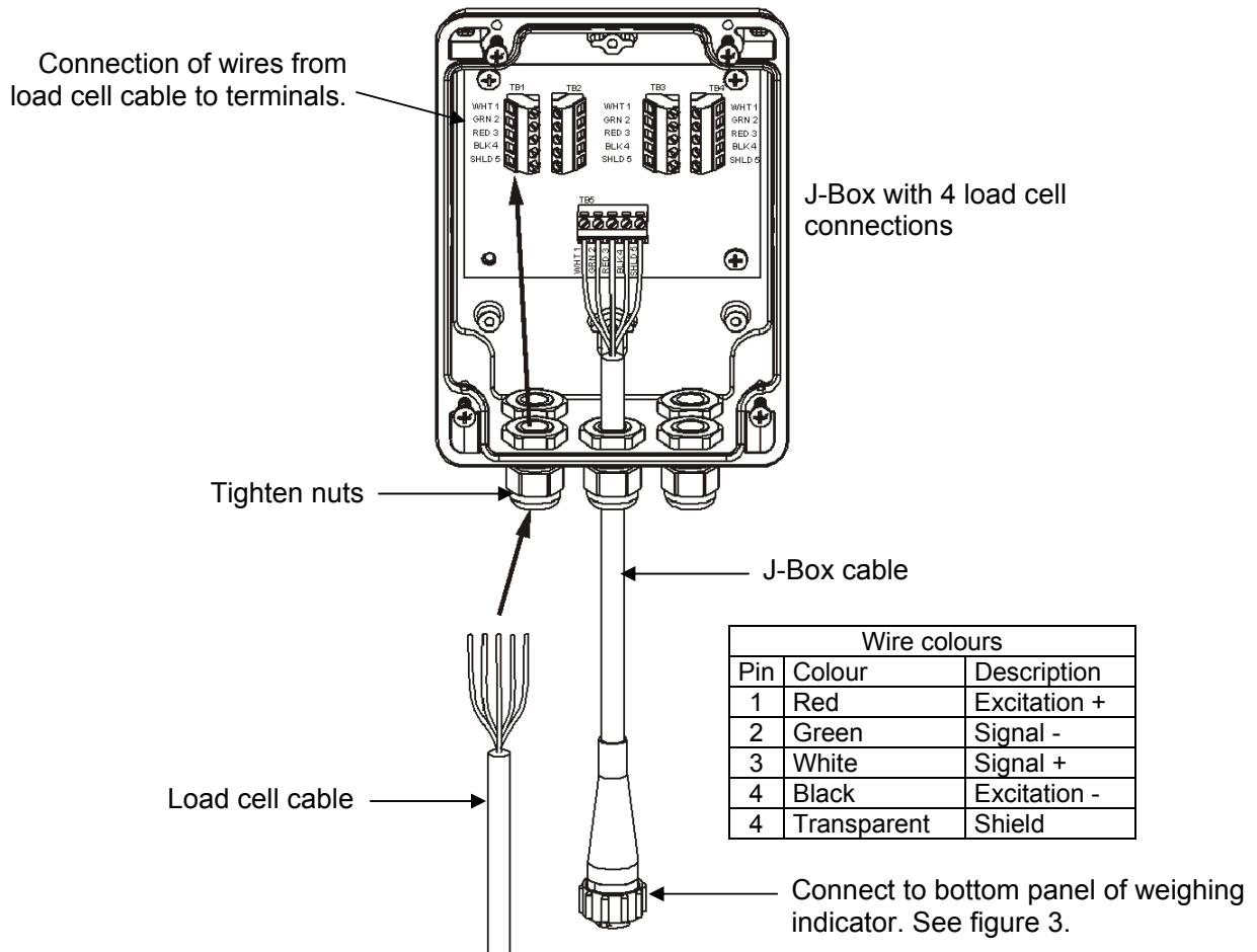
Figure 4: J-Box connections
